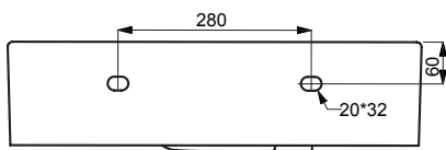
Back view with mounting holes
