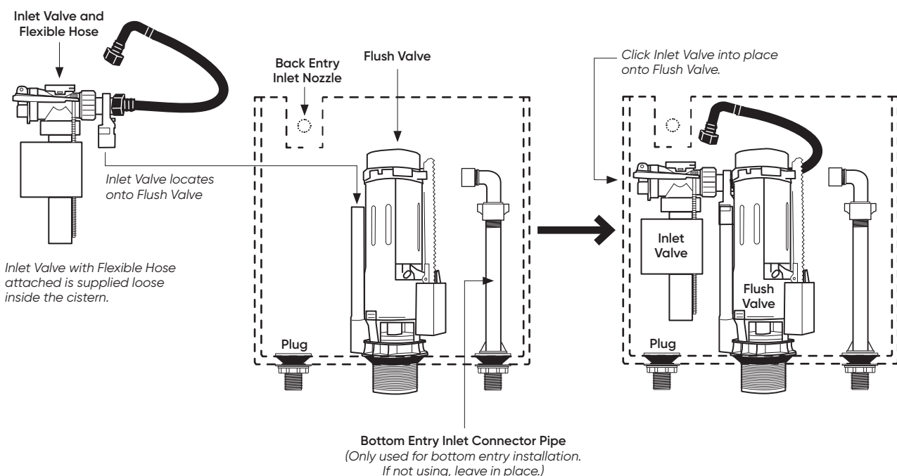
Diagram A – Cistern setup when supplied
