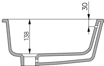
Slot overflow at front of basin
